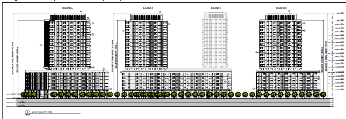
Image 9 - Conceptual elevation (West)
