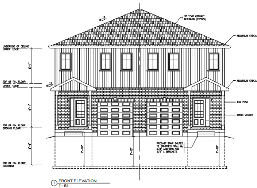
Figure 2: Front Elevation
