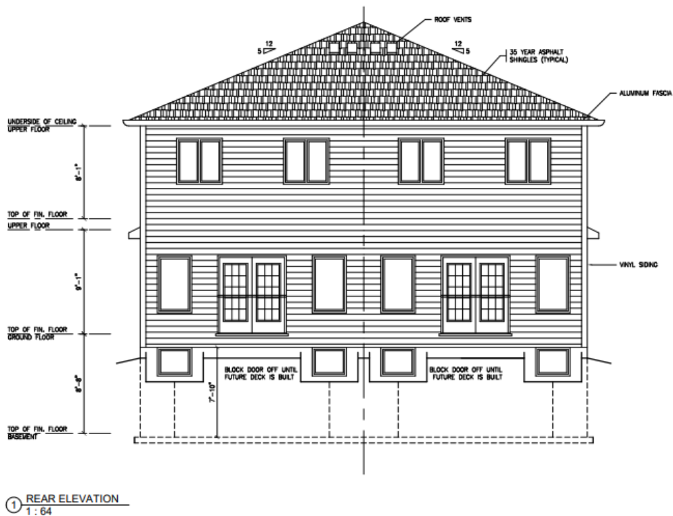
Figure 3: Rear Elevation
