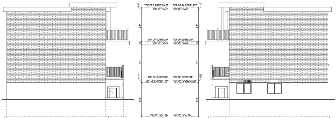
LEFT ELEVATION
